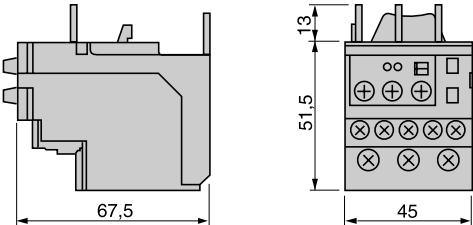
LR97D●●●●
