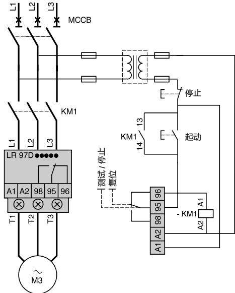
LR97D●●●●
